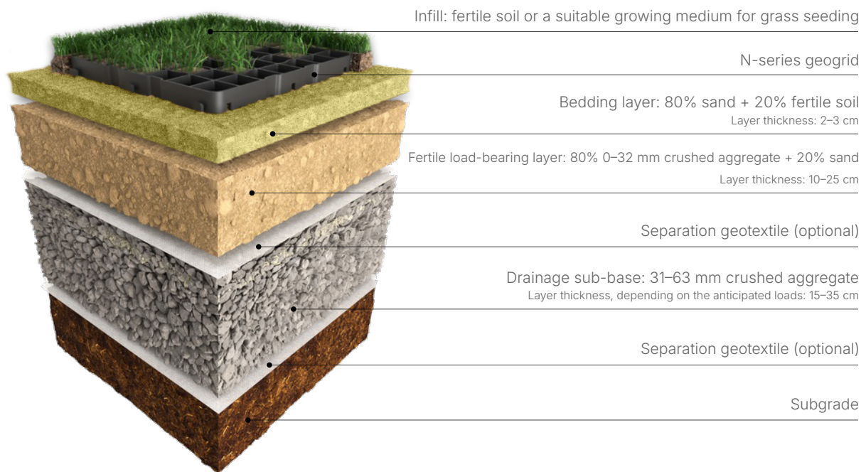
Figure 4 Suggested sub-base build-up
