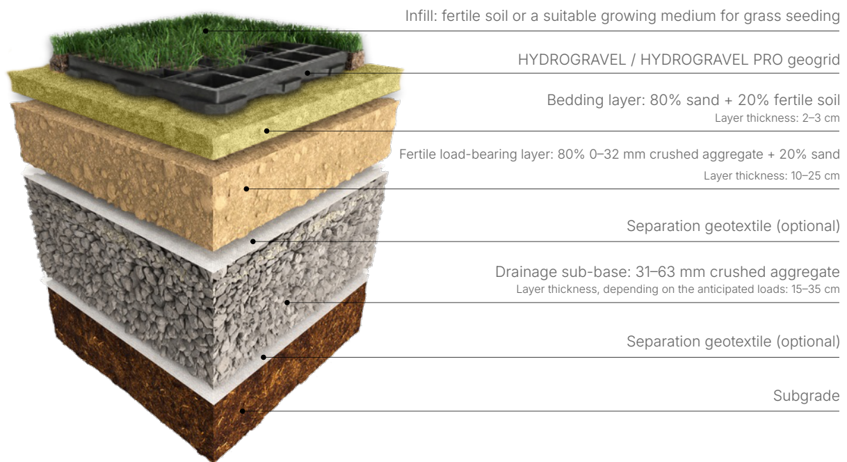
Figure 5 Suggested sub-base build-up
